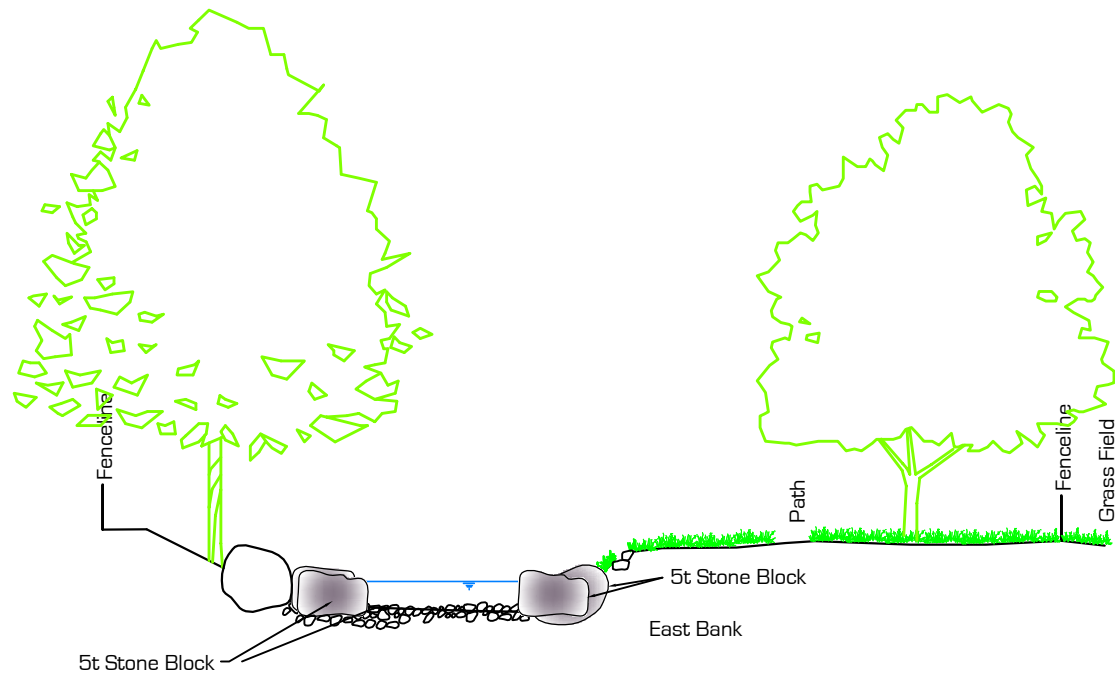
Location C Existing Indicative Section
